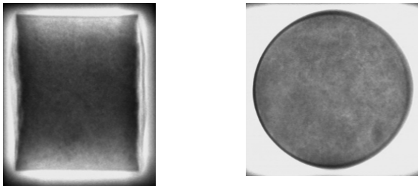
Fig. 9 X-Ray analysis of soil disturbance from KU-miniature sampler
