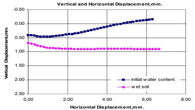
Fig. 11 Change in vertical displacement from SRI test
