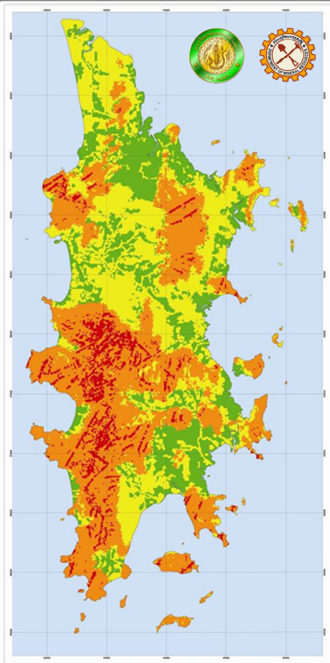
Fig. 19 Landslide hazard map of Phuket considering 1 year return period 3 days accumulated rainfall
