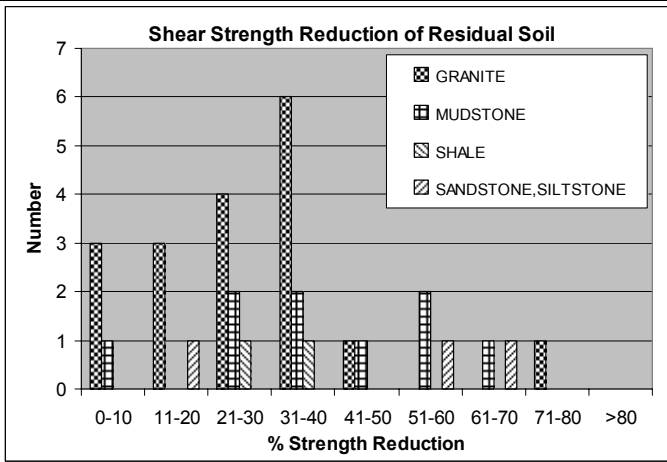
Fig. 13 Percent of shear strength reduction of residual soil of various rock type from SRI test
