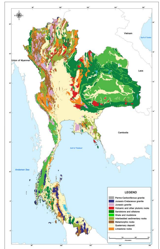
Fig. 5 Landslide rock group of Thailand (Sorarlump, 2007)
