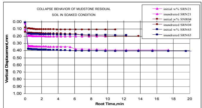
Fig. 12 Collapse behavior of mudstone residual soil after soaked
