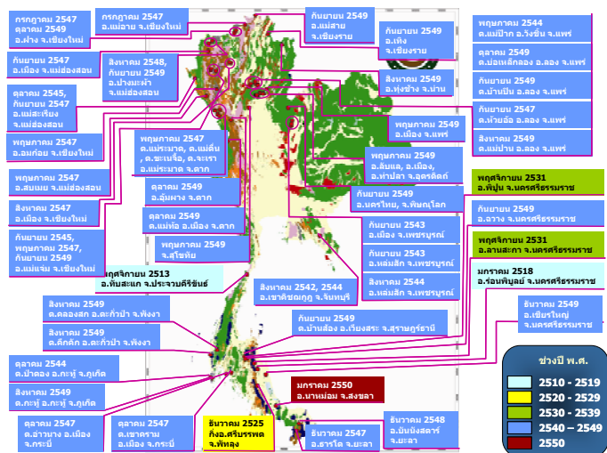
Fig. 1 Landslide events in Thailand (GERD, 2006)
