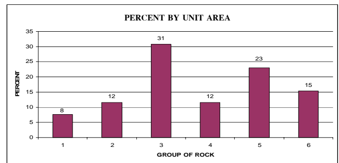
Fig. 6 Number in percent of landslide events in Thailand classified by frequency of occurring in each rock group
