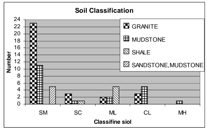
Fig. 15 Soil classification of residual soil
